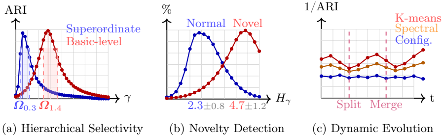
Fig. 4: Brain-inspired capabilities of configurations. (a) Superordinate categories emerge at low \gamma (0.2–0.6), basic-level at high \gamma (1.2–1.8). Plateaus show stable organizational scales. (b) Energy distributions distinguish novel from familiar stimuli (87% AUC), paralleling infant habituation. (c) Configurations achieve stable 35% lower 1/\text{ARI} than other two baselines during category evolution.
